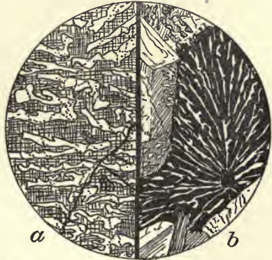
Fig. 25.— a , Graphic Granite. Vein in Stanner Rock, Herefordshire. \times 8 . Nicols crossed. Clear quartz; microcline with characteristic twinning. b , Micropegmatitic intergrowth of quartz and feldspar, in Eurite. Stanner Rock, Herefordshire. \times 160 . Nicols crossed. The feldspar is in a position of extinction. Other micropegmatitic areas and feldspar crystals lie around.
